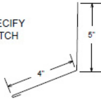
ENDWALL FLASHING
